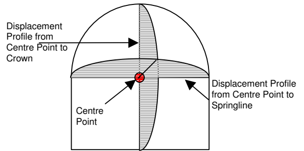
Figure 5: Idealised Displacement Profiles on the Tunnel Face.
